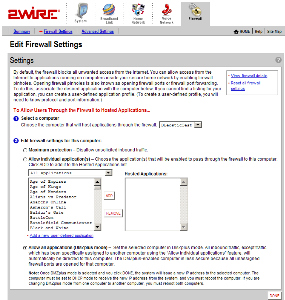
Figure 20. Edit Firewall Settings Page
